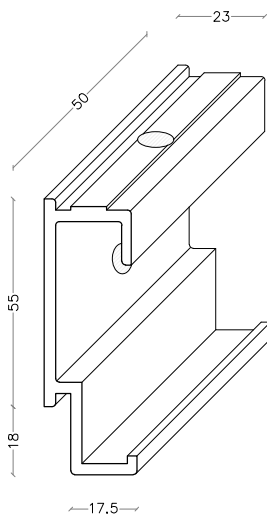
Horizontal Rail Top Clip
