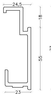
Horizontal Support Rail
