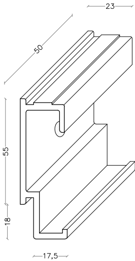
Horizontal Rail Bottom Clip
