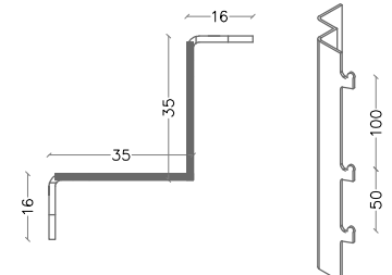
Vertical Corner Support Profile (250mm)
