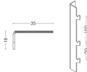
Vertical Support Profile (250mm)
