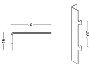
Vertical Support Profile (200&300mm)
