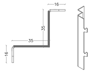
Vertical Corner Support Profile (200&300mm)
