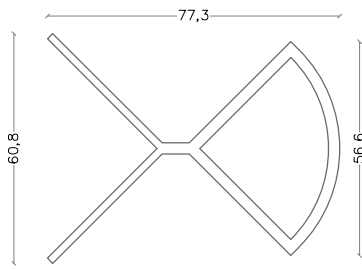
Closed Corner Profile
