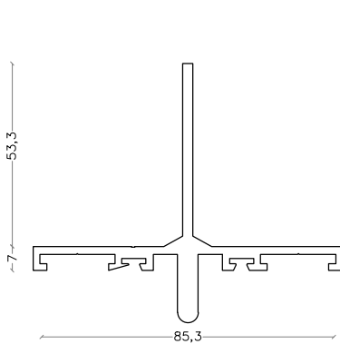
Channel T Profile
