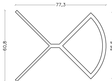
Closed Corner Profile
