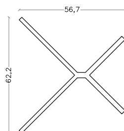
Open Corner Profile
